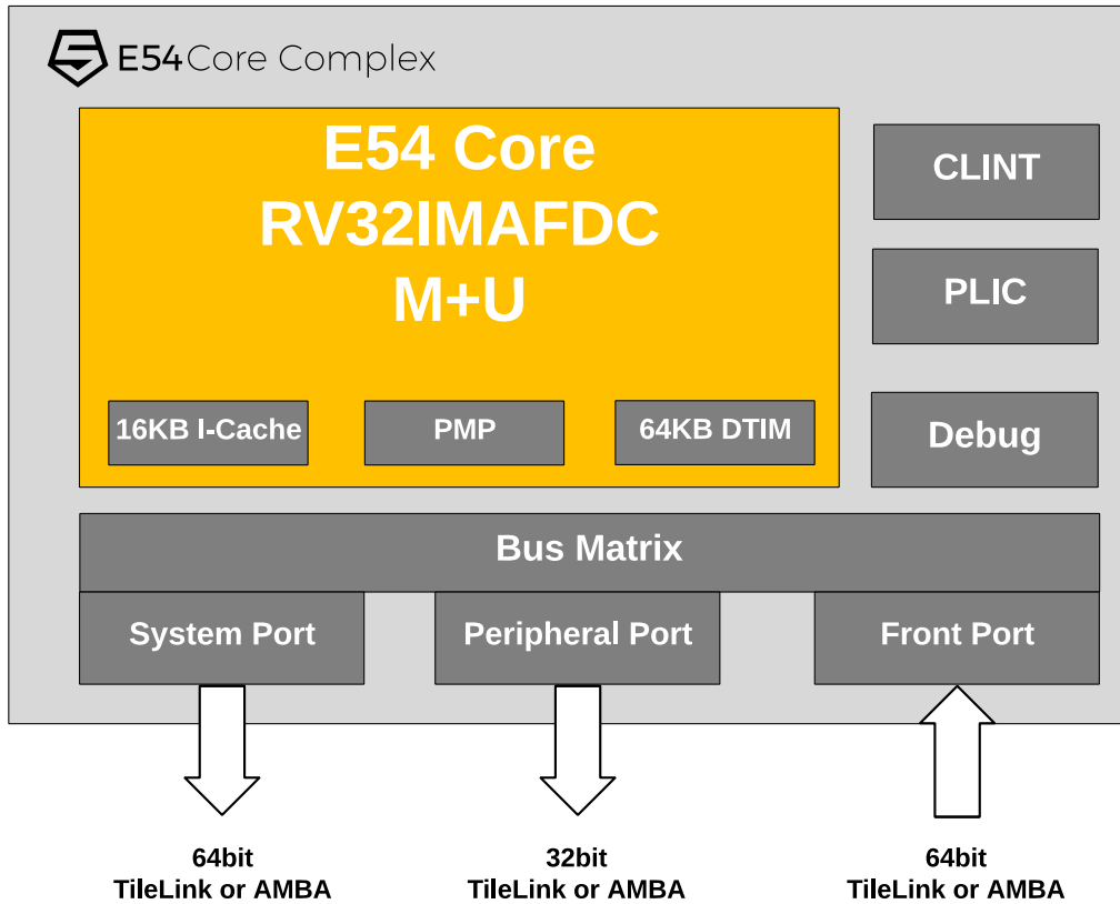
Figure 1: E54 Core Complex Block Diagram
